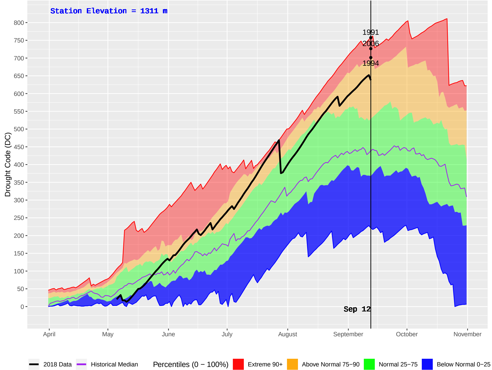
FLATHEAD 2 (418) : Historical (1986–2016) and Current (2018) Daily Drought Code (DC)
