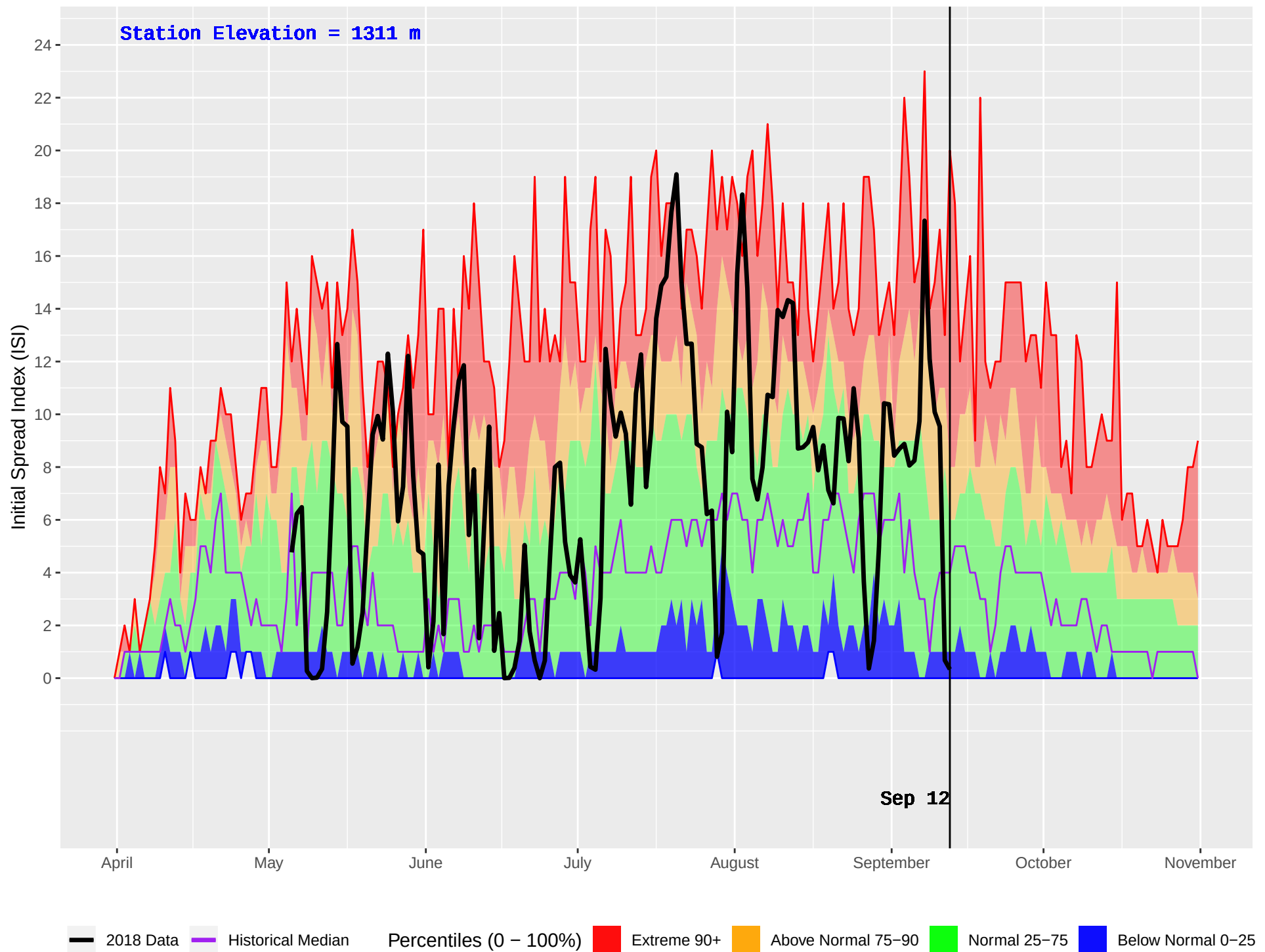
FLATHEAD 2 (418) : Historical (1986–2016) and Current (2018) Daily Initial Spread Index (ISI)
