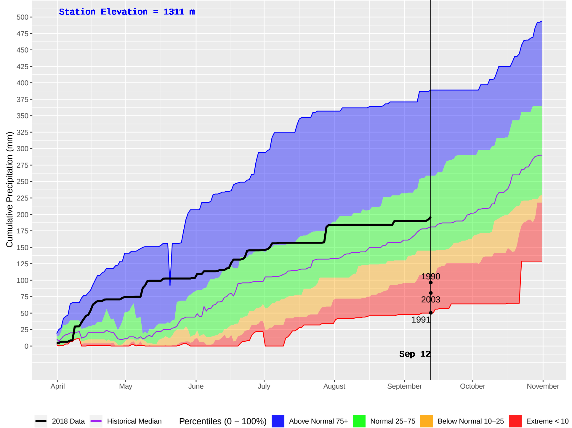
FLATHEAD 2 (418) : Historical (1986–2016) and Current (2018) Daily Cumulative Precipitation
