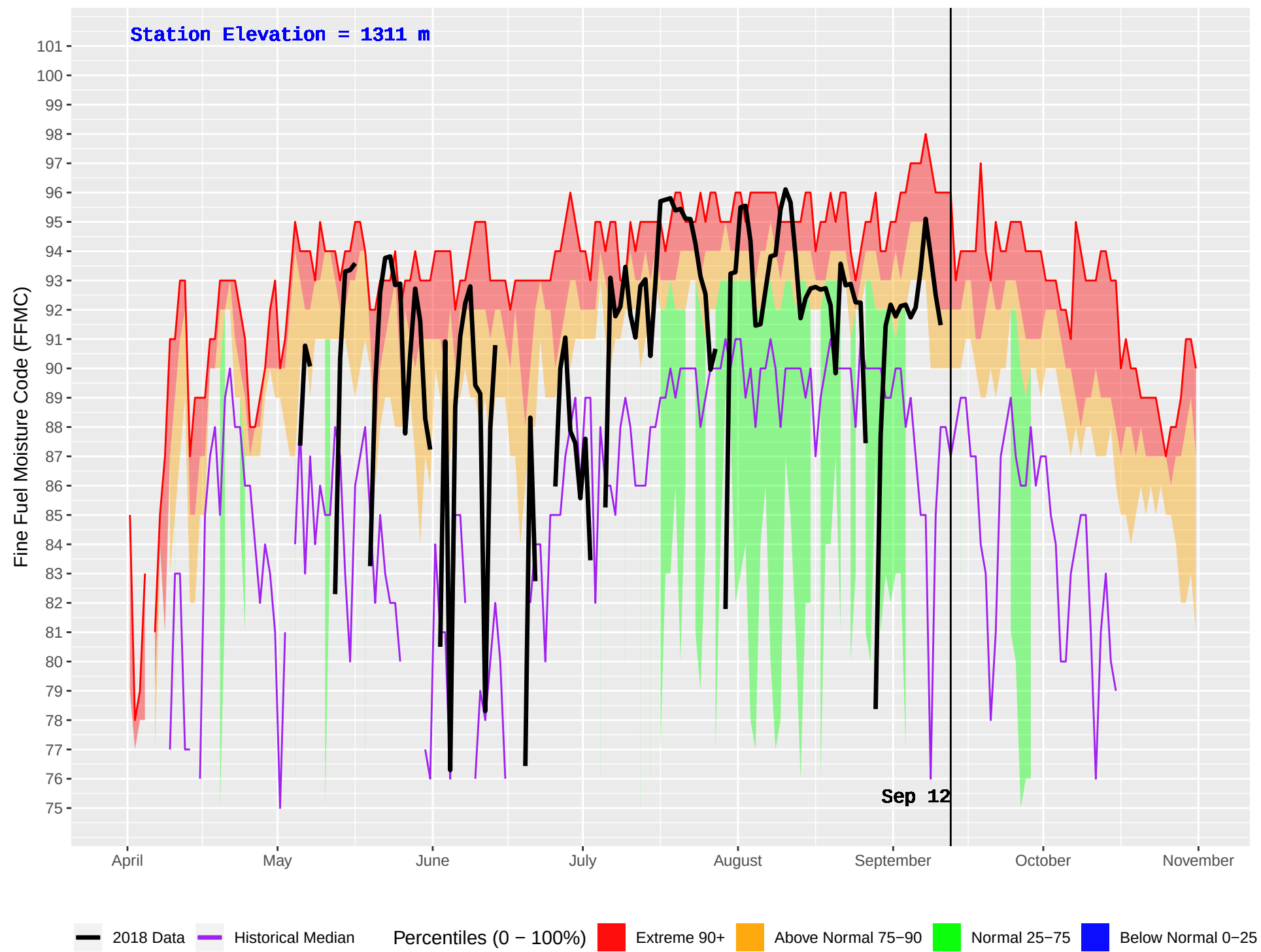
FLATHEAD 2 (418) : Historical (1986–2016) and Current (2018) Daily Fine Fuel Moisture Code (FFMC)
