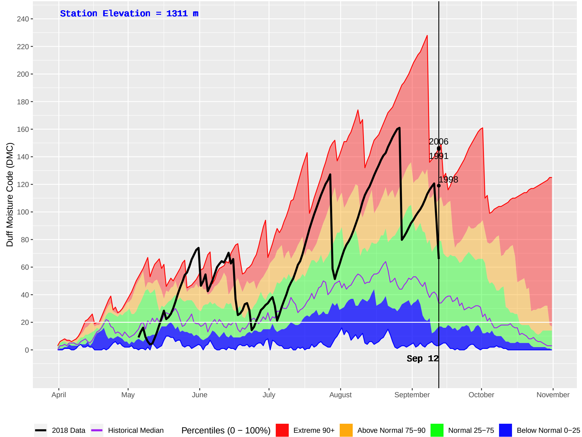
FLATHEAD 2 (418) : Historical (1986–2016) and Current (2018) Daily Duff Moisture Code (DMC)
