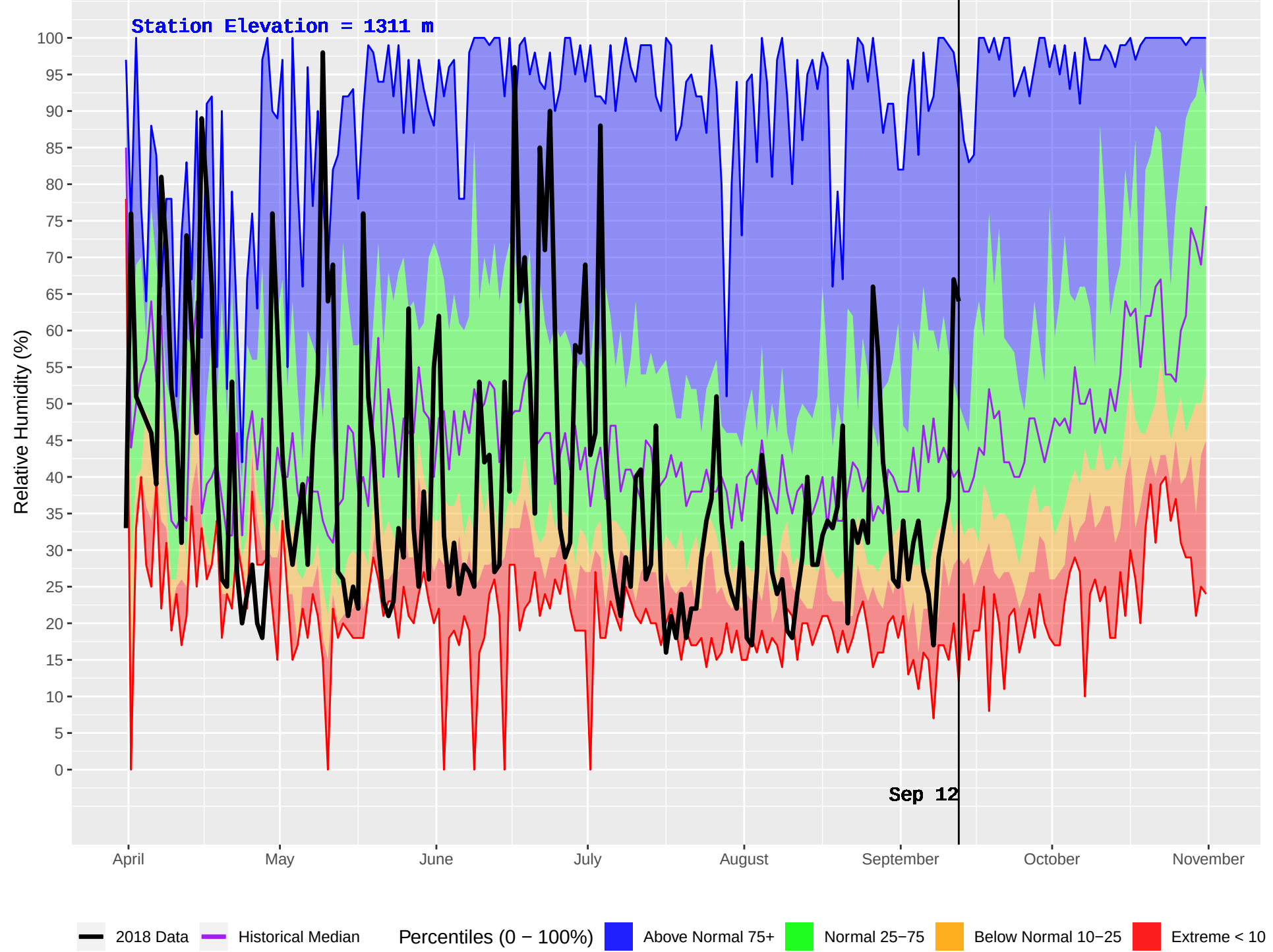
FLATHEAD 2 (418) : Historical (1986–2016) and Current (2018) Daily Relative Humidity
