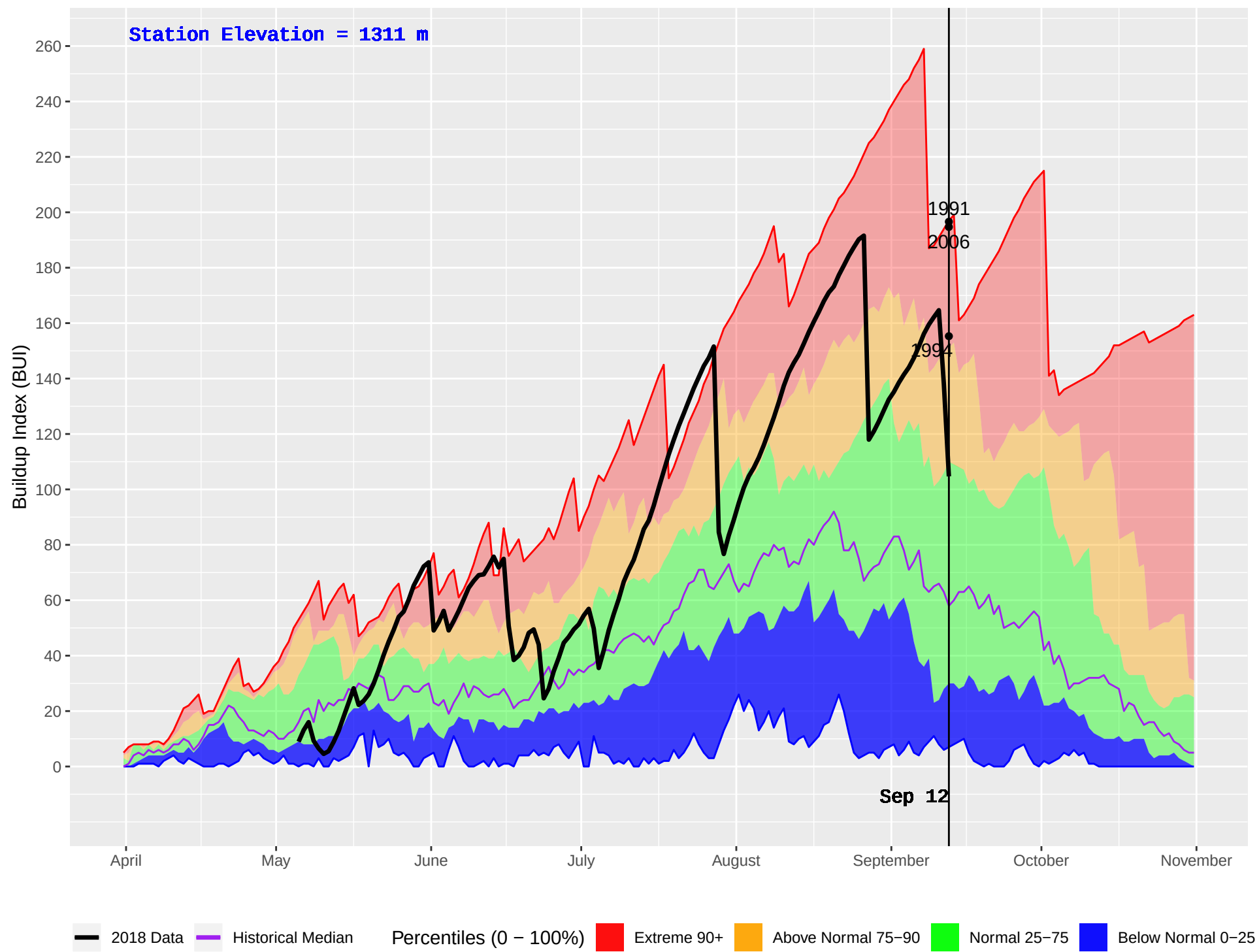
FLATHEAD 2 (418) : Historical (1986–2016) and Current (2018) Daily Buildup Index (BUI)
