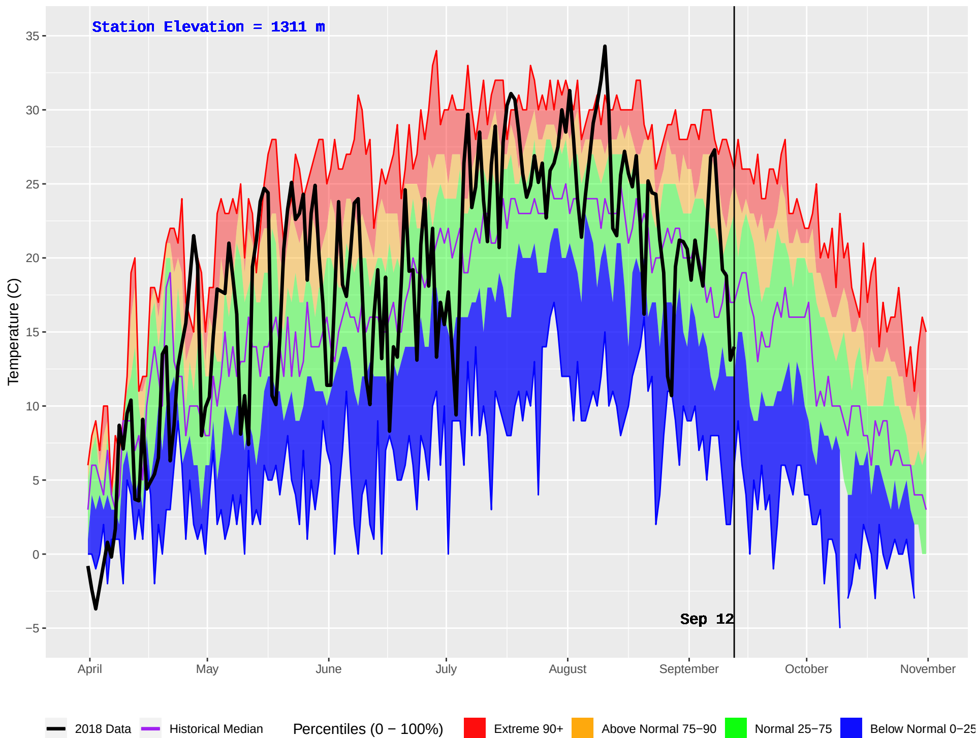
FLATHEAD 2 (418) : Historical (1986–2016) and Current (2018) Daily Temperature
